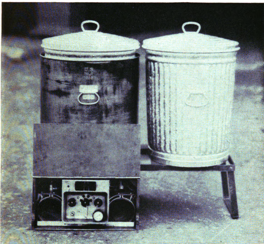
FIGURE 35.—Water heater set up for use (case, can, can cover, and can shield).
